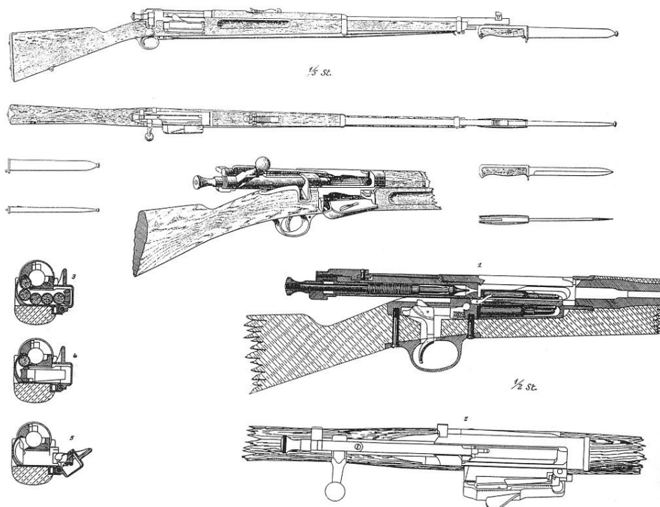
Krag-Jørgensen's Gevær. Model 1892.
