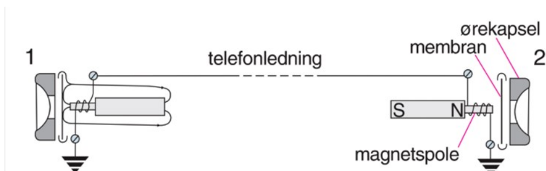
Prinsippet for Bells telefon.
